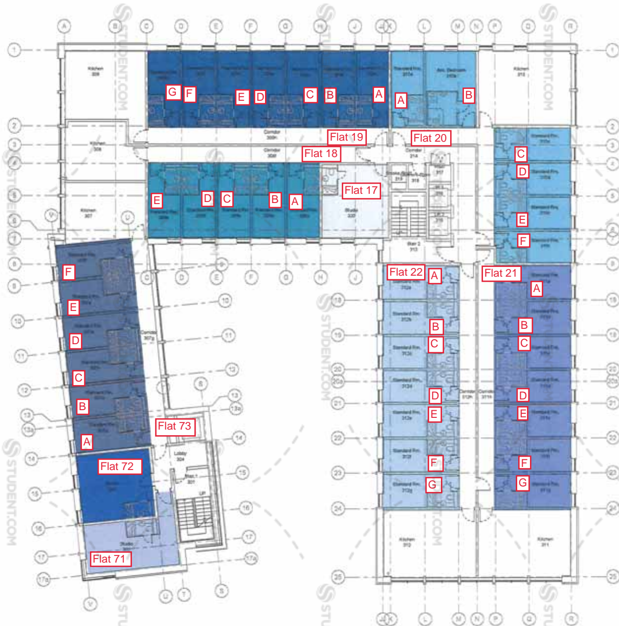
1 GA Floor Plan - Postal Address Layout - Level 3 1:100
